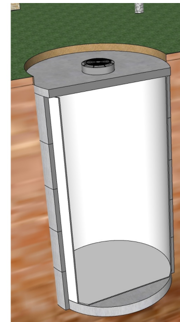
7. Place RC Slab, Install Frame & Cover
