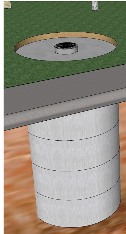
Installed Cistern
