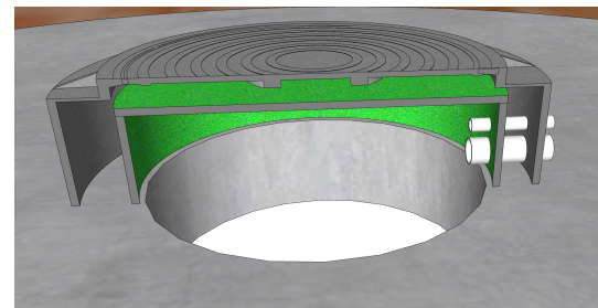
Frame and Cover Detail
